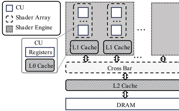
Figure 1: A general purpose GPU memory hierarchy. Arrows indicate data-flow paths.
