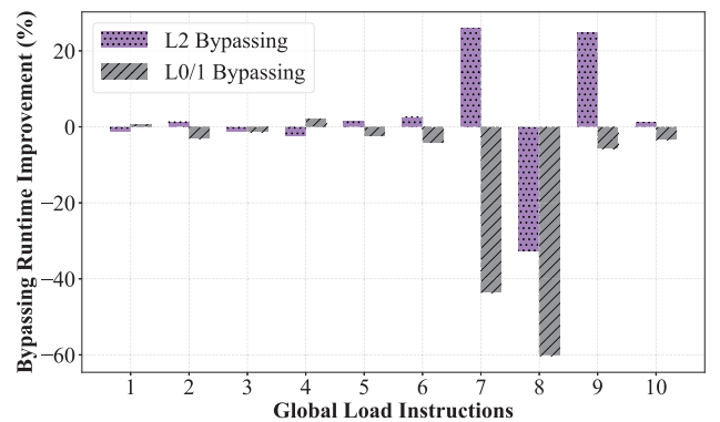
Figure 2: The percentage of runtime improvement of spmv for bypassing each load under L2 Bypassing mode and L0/1 Bypassing mode.
