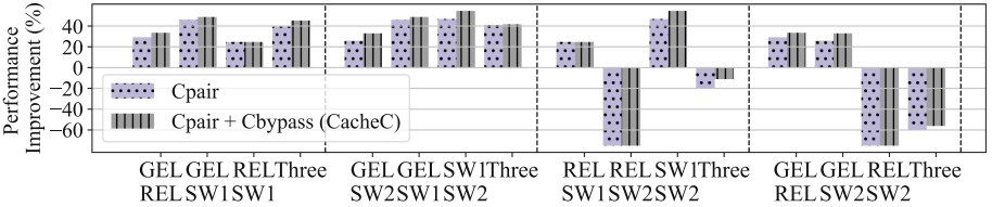
Fig. 8. Performance gains of Cpair and CacheC over Baseline for three-kernel execution and all two-kernel combinations from the three kernels.
